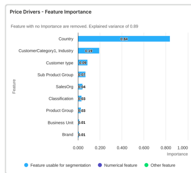
Feature Importance
