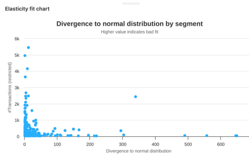
Elasticity fit chart
