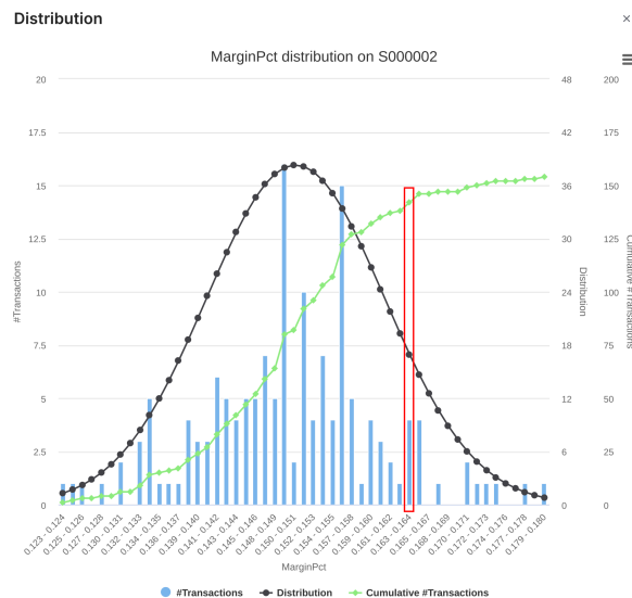
Histogram of data for segment S000002
