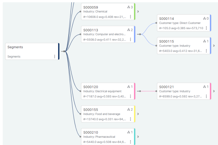
Segmentation tree for the alignment example
