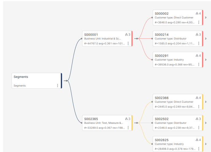
Segmentation tree for price gaps example
